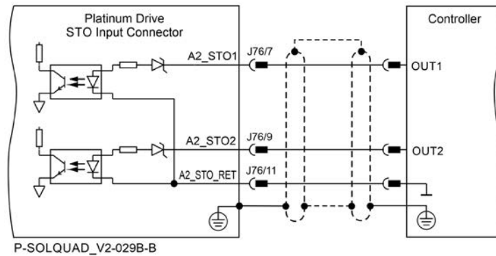
Figure 19: STO Shrouded Type Input Connection – PLC Source Option for Axis A2
