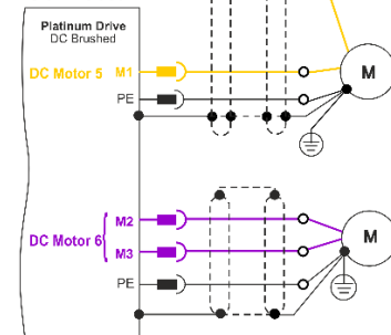
Figure 14: 6-Axis Brushed Motor Power Connections Diagram
