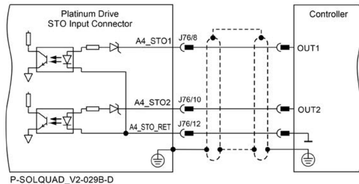
Figure 21: STO Shrouded Type Input Connection – PLC Source Option for Axis A4
