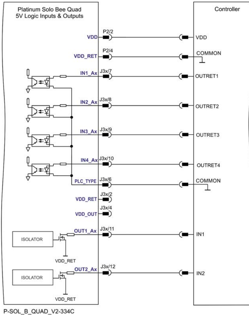
Figure 34: Regular Digital Input and Output 5V Logic Mode Connection Diagram
