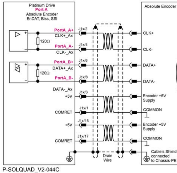
Figure 27: Absolute Serial Encoder – Recommended Connection Diagram for EnDat, Biss, SSI
