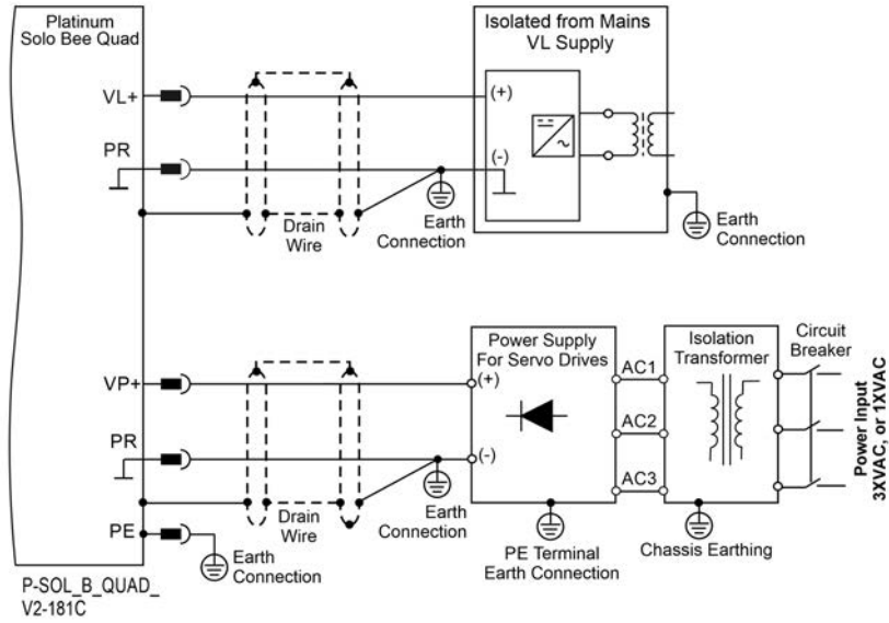
Figure 15: Power Supply Connection Diagram for Power Rating 200V
