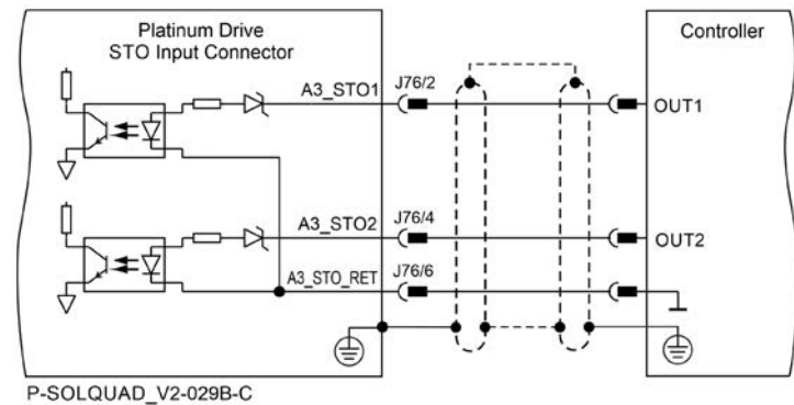
Figure 20: STO Shrouded Type Input Connection – PLC Source Option for Axis A3
