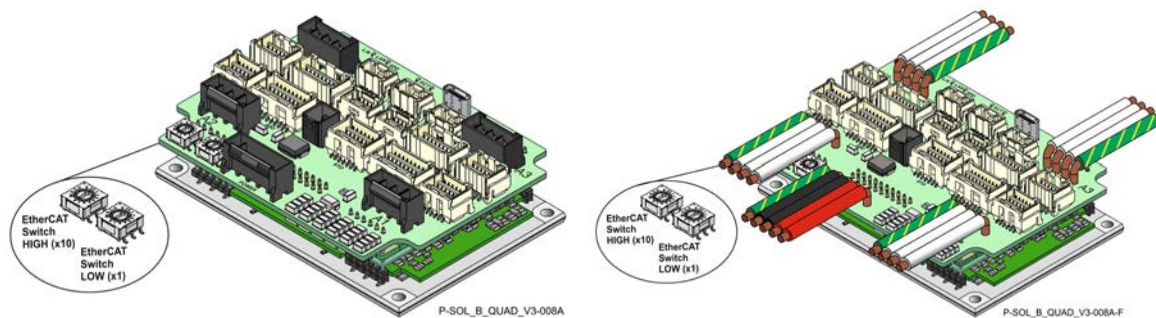
Figure 42: EtherCAT Address Switches
