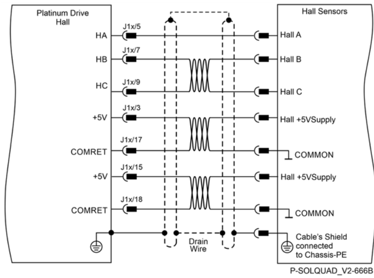
Figure 31: Hall Sensors Connection Diagram
