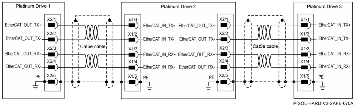
Figure 39: EtherCAT Schematic Diagram for Platinum to Platinum drive connections
