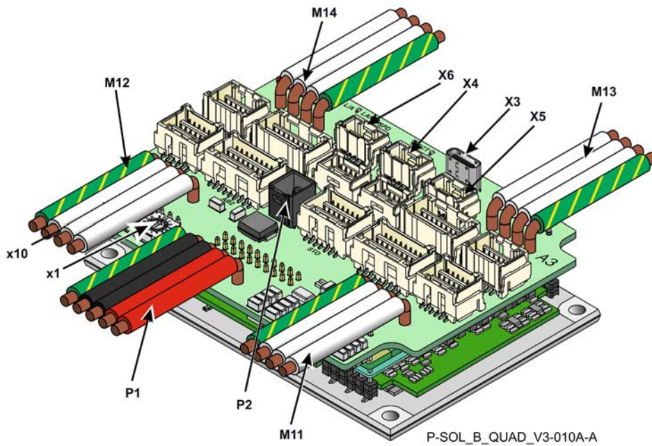
Figure 4: Wired Power Connection Names and Locations
