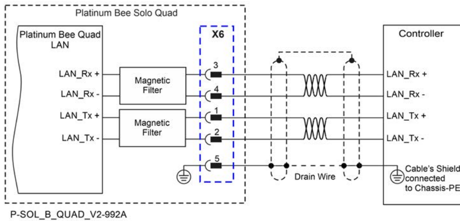
Figure 43: EtherCAT Connection Schematic Diagram
