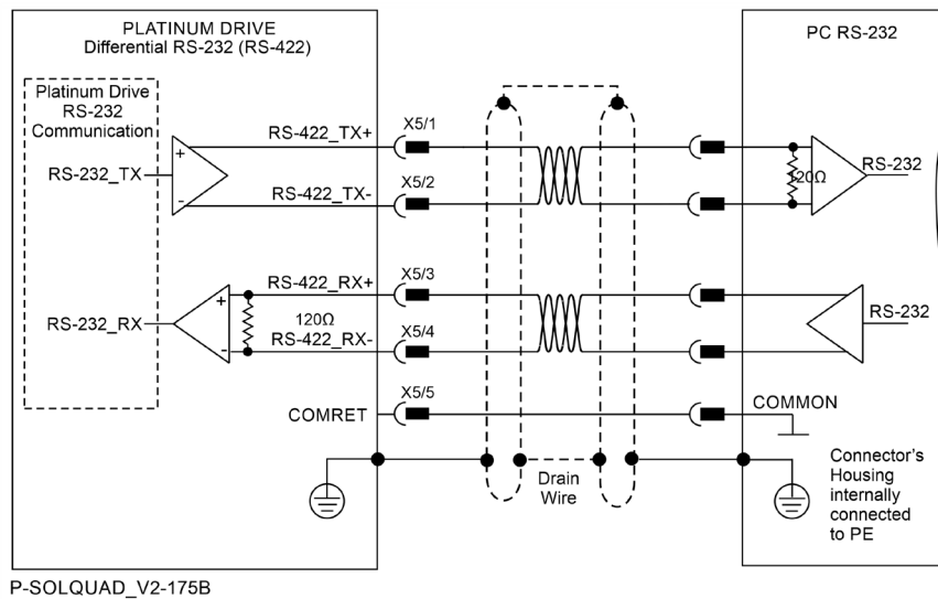
Figure 38: Differential RS-232 Communication Example for Connector X5
