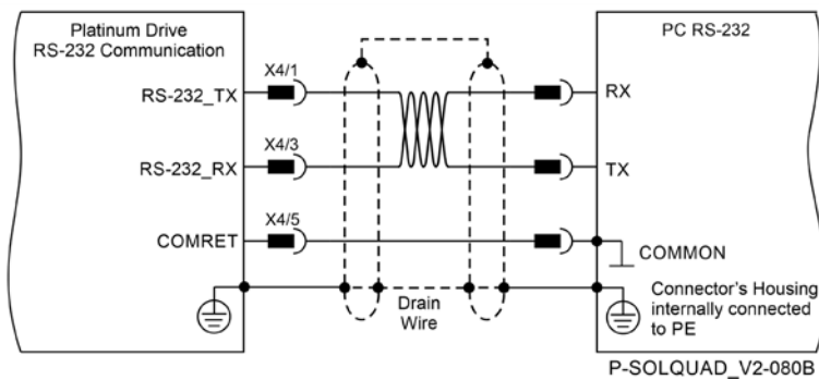
Figure 37: RS-232 Connection Diagram
