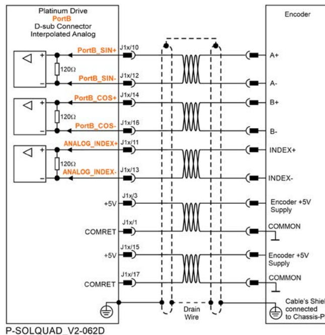
Figure 30: Port B - Interpolated Analog Encoder Connection Diagram
