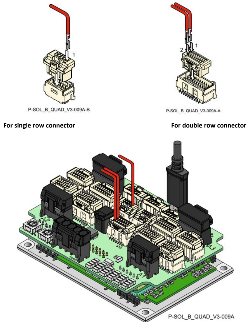
Figure 12: Inserting a wire/pin to the Female CON CLIK-MATE Connector
