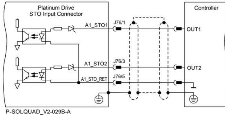
Figure 18: STO Shrouded Type Input Connection – PLC Source Option for Axis A1
