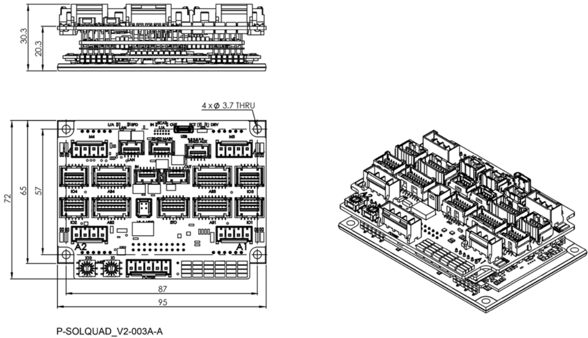
Figure 45: Platinum Solo Bee Quad with Power and Motor Connectors
