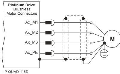
Figure 13: 4-Axis Brushless Motor Power Connection Diagram
