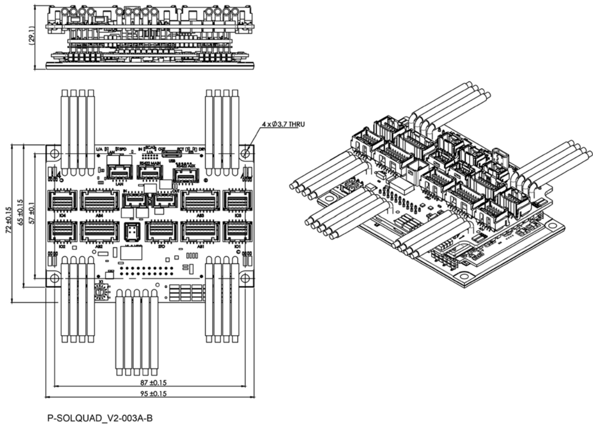
Figure 46: Platinum Solo Bee Quad with Power and Motor Wires
