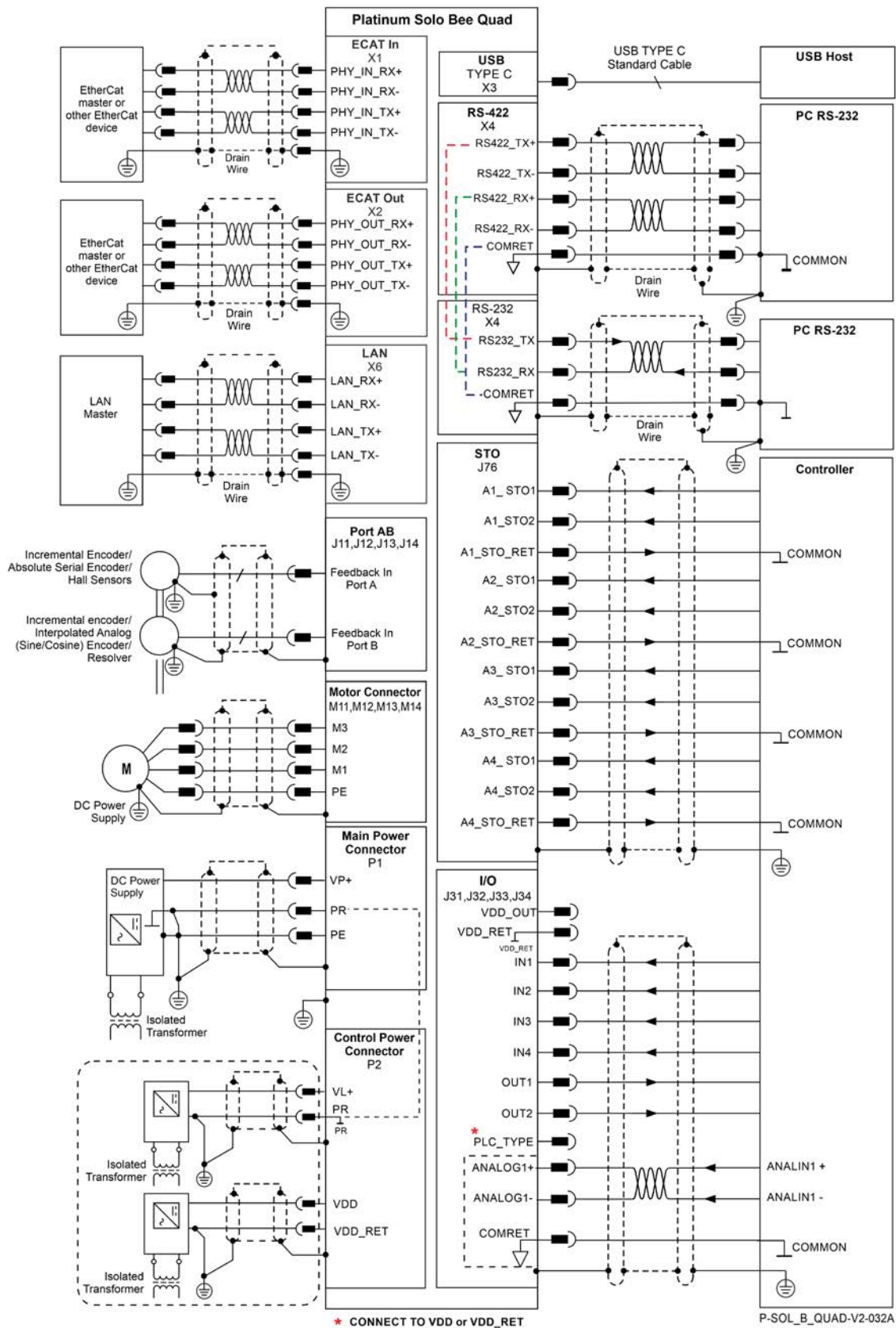
Figure 11: Platinum Solo Bee Quad EtherCAT Connection Diagram
