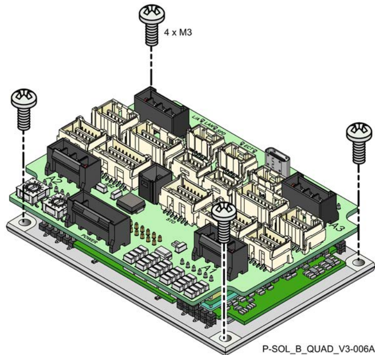
Figure 2: Mounting the Platinum Solo Bee Quad
