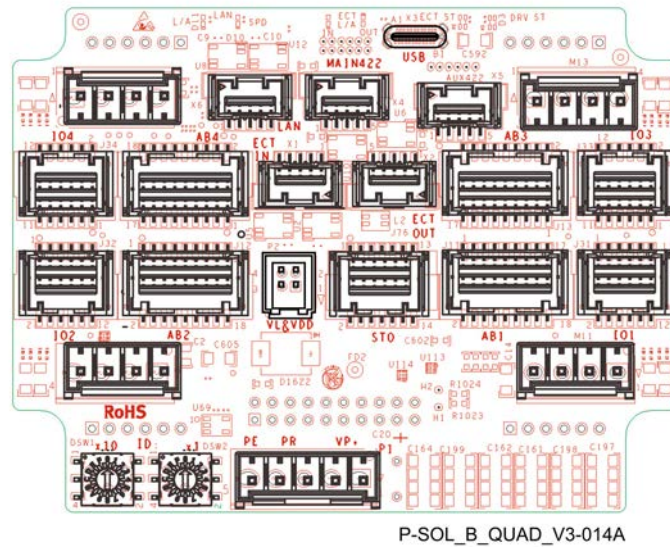
Figure 8: Platinum Solo Bee Quad Board Indicator Labelling
