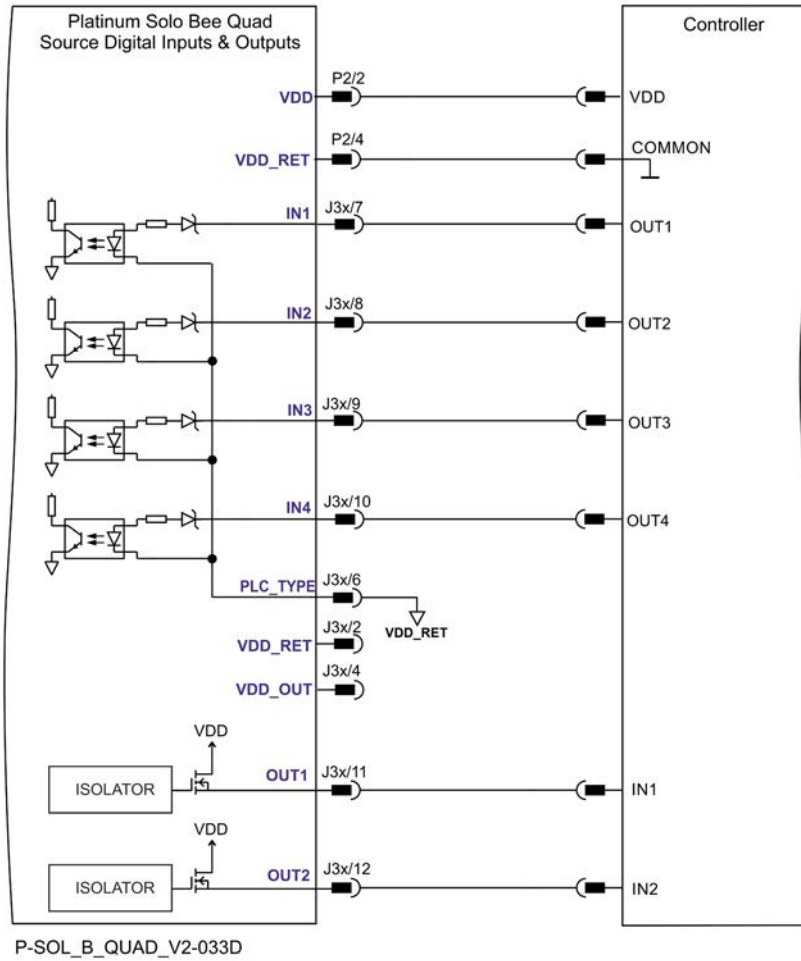
Figure 32: Digital Input and Output Connection Diagram – Source PLC Option
