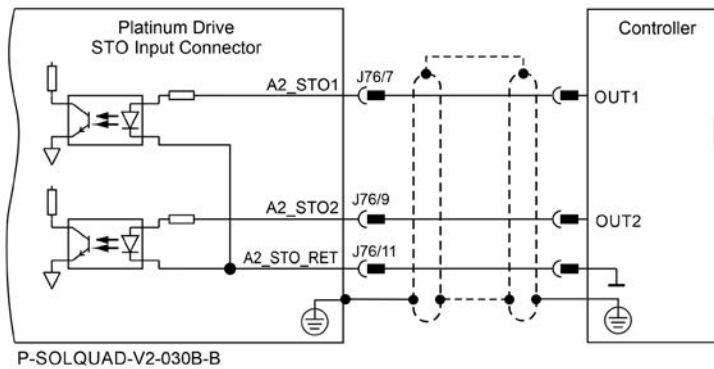
Figure 23: STO Input Connection – TTL Option for Axis 2
