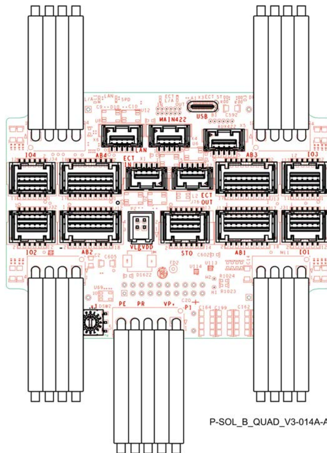
Figure 9: Platinum Solo Bee Quad Board Indicator Labelling (Wired Power Connection)
