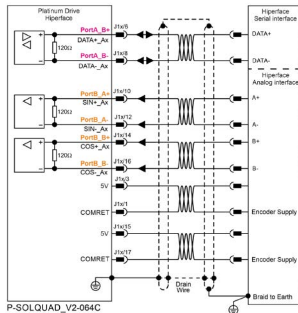
Figure 28: Absolute Serial Encoder – Recommended Connection Diagram for Stegmann Hiperface
