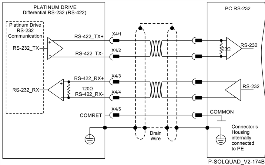
Figure 36: Differential RS-232 Communication Example for Connector X4
