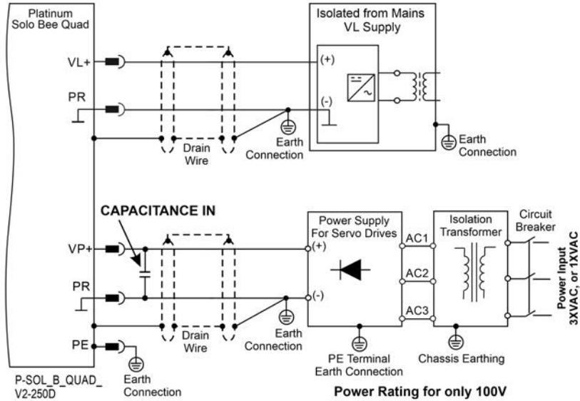
Figure 17: Shared Optional Power Supply Connection Diagram
