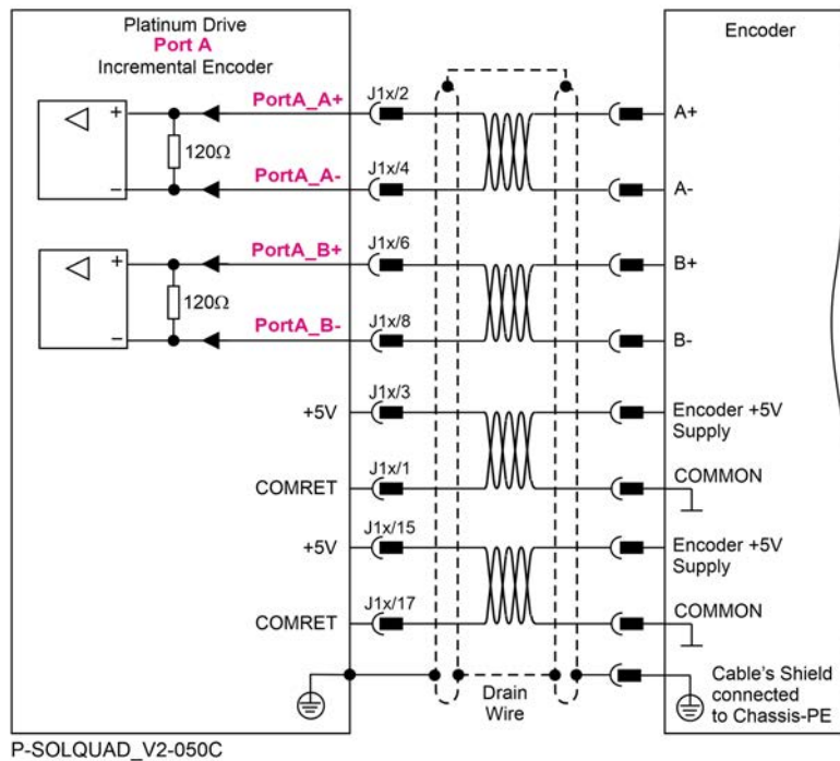
Figure 26: Port A Incremental Encoder Input – Recommended Connection Diagram
