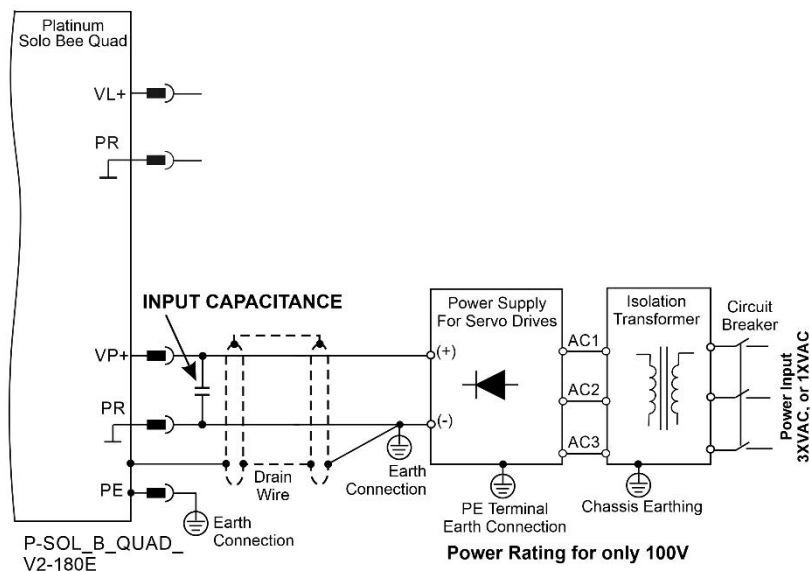
Figure 16: Main Power Supply Connection Diagram (No Control Supply)
