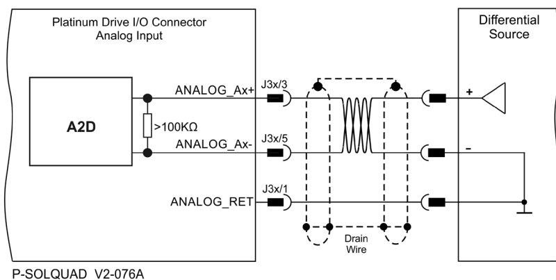
Figure 35: Differential Analog Input
